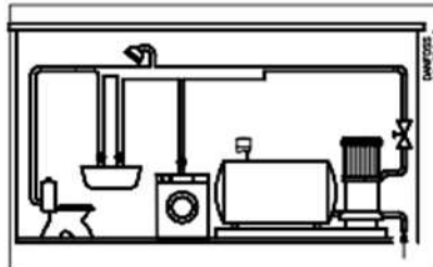
Example 5 Pressure boosting system for domestic circuits. A type CS switch is used to start/stop the pump.
